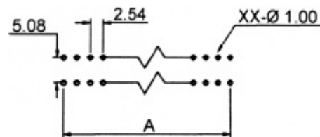
PC Board Layout 36, 62 Pins
