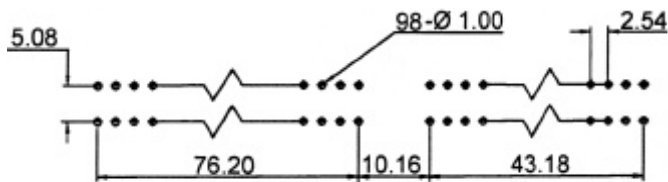
PC Board Layout 98 Pins
